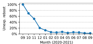
Figure 9: Unexpected VM reboot.
