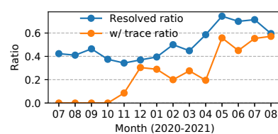
Figure 11: Ticket resolved and w/ trace ratio.
