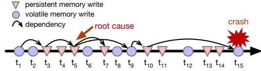
Figure 6: Timeline of volatile and persistent memory writes.
