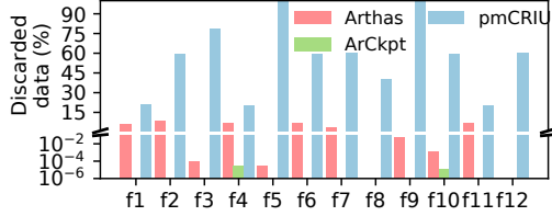
Figure 9: Data discarded in rollback by different solutions.
