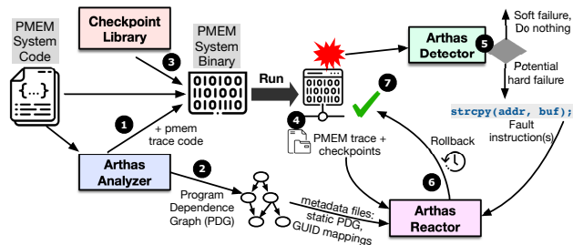
Figure 4: Overview of Arthas design.
